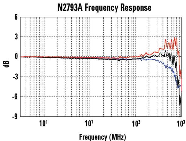
Figure 10. V_{out}/V_{in} vs. Frequency response of N2793A /N2819A (red = V_{out}/V_{in} , blue = V_{in} , black = V_{out} )
